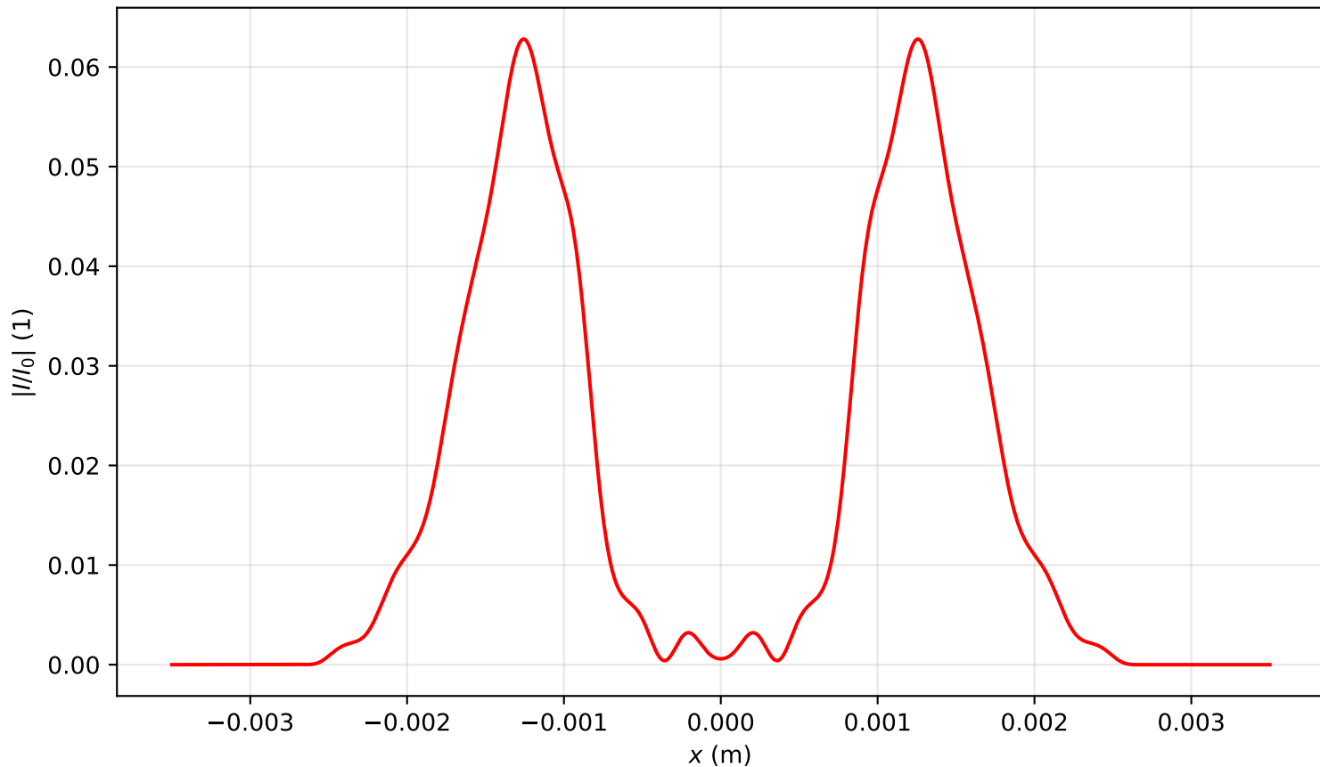
Intensity profile I(x, y = 0, z = 3.821)/I_0 , P_{in}=6.5P_{cr} , artificial time
